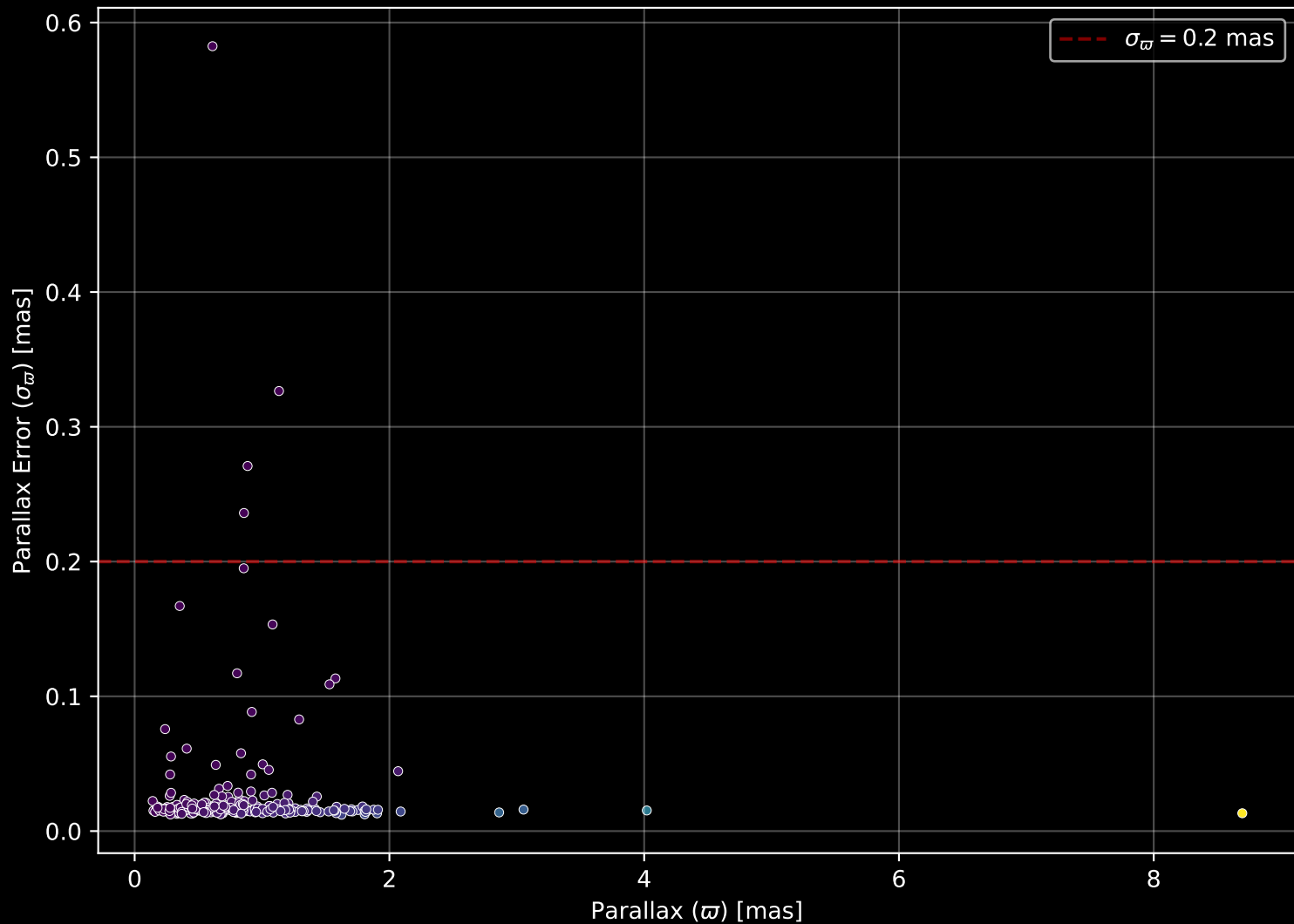
GALAH DR4 Field: [9277] Parallax Quality (n= 258)
