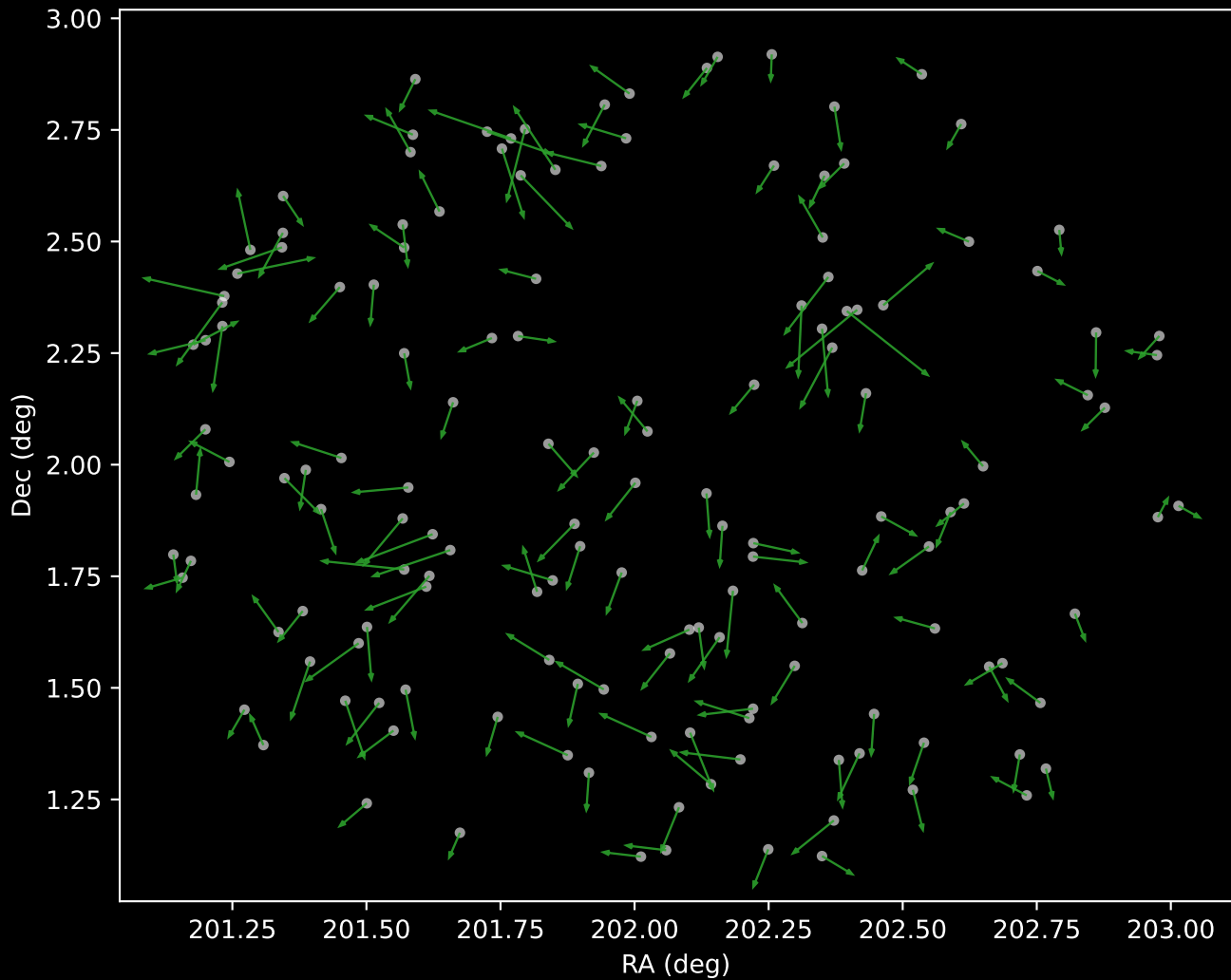
GALAH DR4 Cluster 4 Proper Motion Vectors (n=150)
