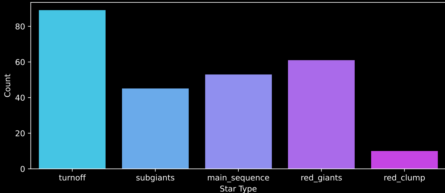
GALAH DR4 Field: [9277] Count plot of Star Type
