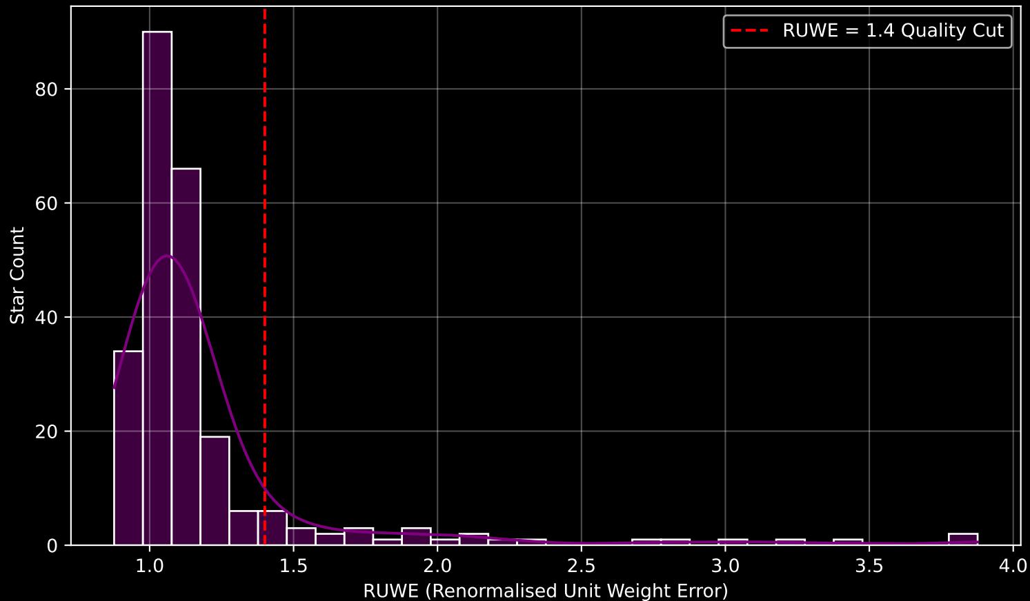
GALAH DR4 Field [9277] RUWE Distribution (n= 245)
