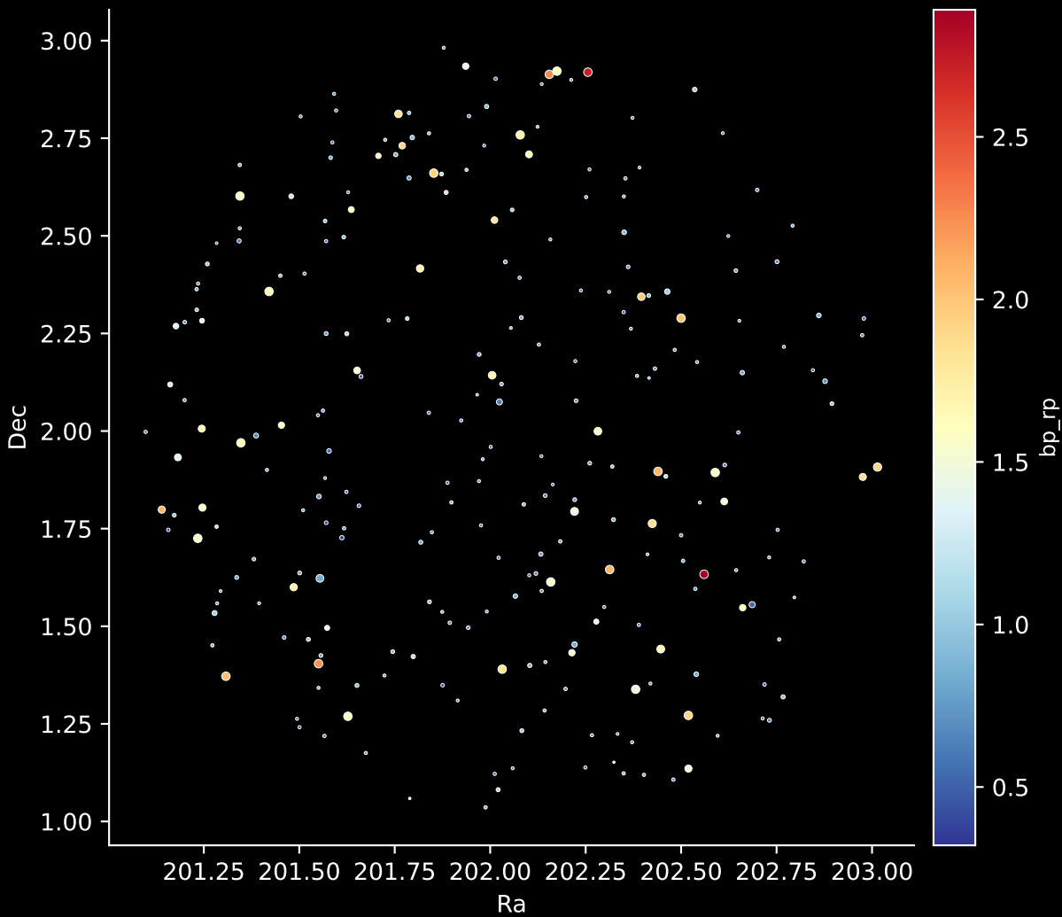
GALAH DR4 Field: [9277] Stars: 258
