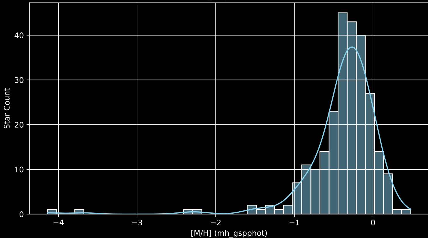
GALAH DR4 Field: [9277] [M/H] (mh_gspphot) (n= 257)
