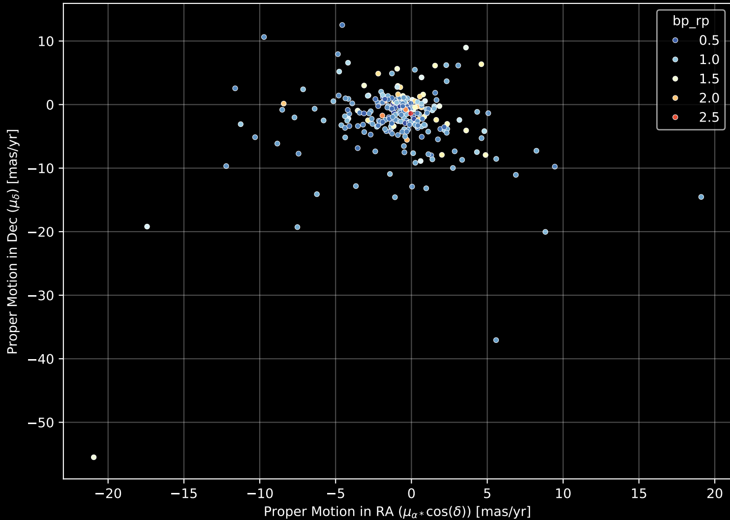
GALAH DR4 Field: [9277] Proper Motion Diagram (n= 258)
